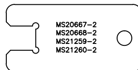
EXAMPLE OF STAMPING FOR G689-01
