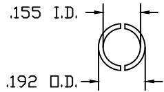
VIEW A
